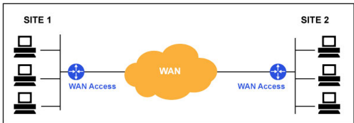
Figure 3: Path Components
