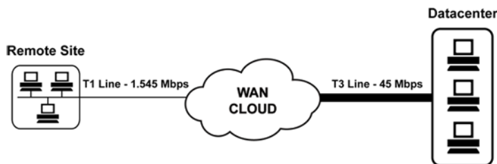
Figure 5: Cloud Network
