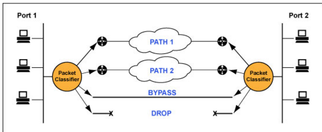
Figure 32: Packet Classification
