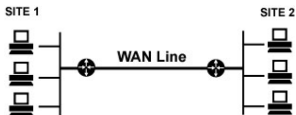
Figure 4: Point-to-Point Line
